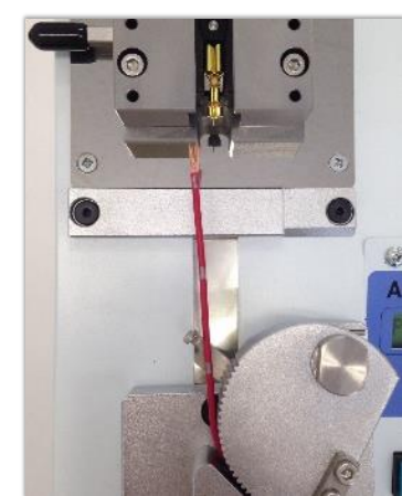
Wire clamping starts as the clammer moves back.
